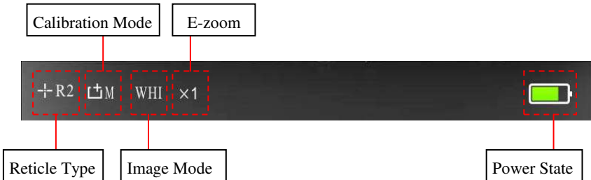
Fig.15 status bar
